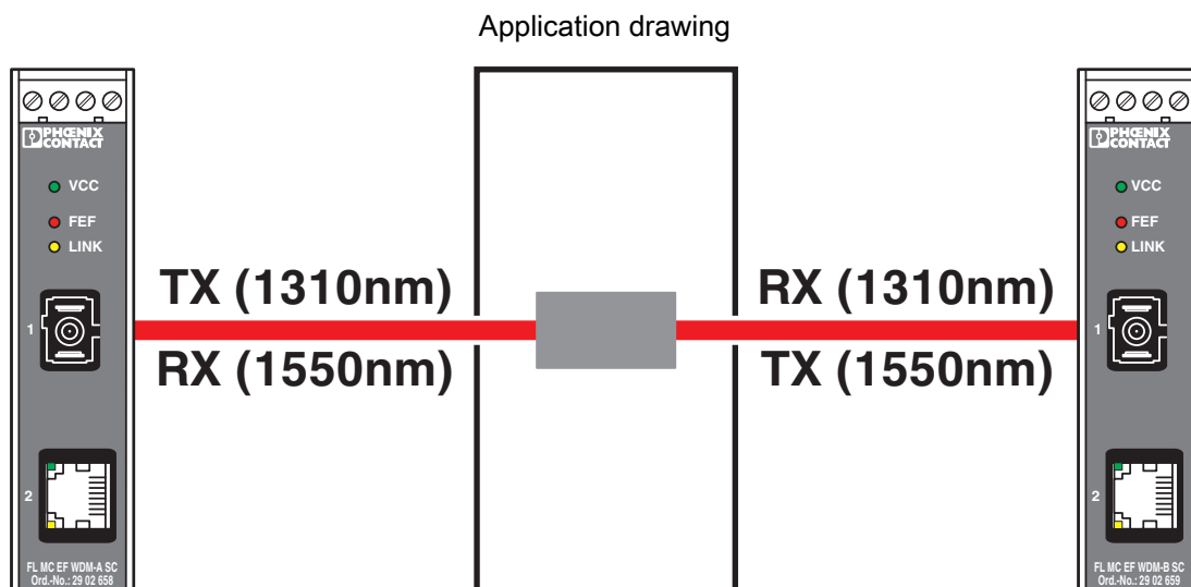
Slip ring communication
